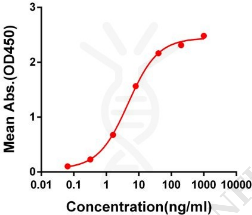
Figure 1. Elisa plate pre-coated by 2 \mu\text{g/ml} (100 \mu\text{l/well} ) SARS-CoV-2 RBD protein can bind Rabbit Anti-SARS-CoV-2 RBD monoclonal antibody ( clone:DM54 ) in a linear range of 0.1-100 ng/ml.
