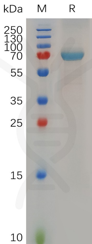
Figure 1. Human B4GALT1, N-hFc Tag on SDS-PAGE under reducing condition.
