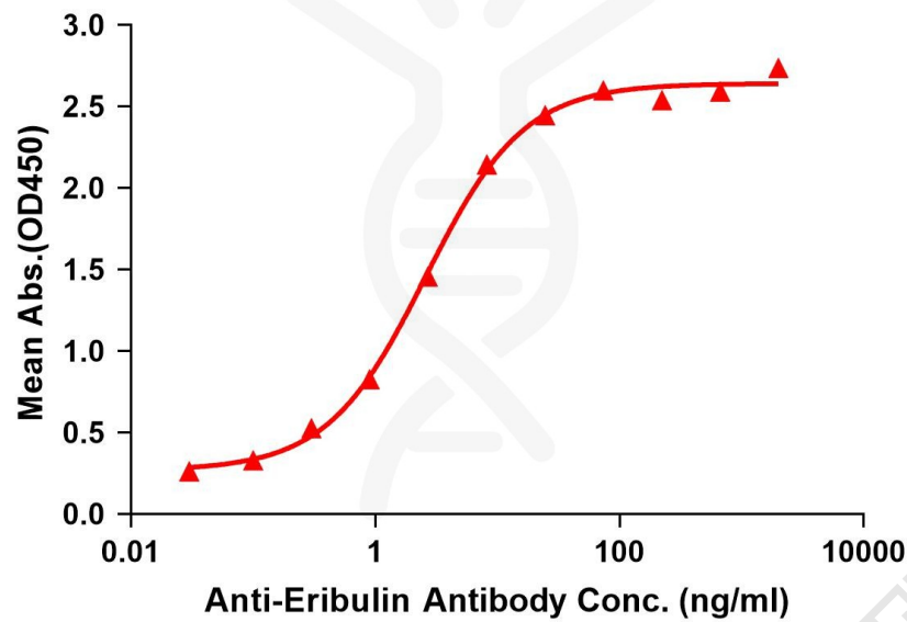
Figure 1. Elisa plates were pre-coated with IgG-Eribulin (0.2µg/per well). Serial diluted anti-Eribulin monoclonal antibody (DME101048) solutions were added, washed, and incubated with secondary antibody before Elisa reading. From above data, the EC50 for anti-Eribulin monoclonal antibody binding with IgG-Eribulin is 2.587ng/ml.
