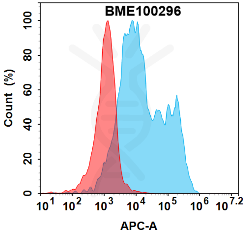
Figure 1. Flow cytometry analysis with 0.5 \mu\text{g/ml} Anti-IL11RA(LASN-01 biosimilar) mAb (BME100296) on HEK293 cells transfected with Human IL11RA protein (Blue histogram) and HEK293 transfected with irrelevant protein (Red histogram) .
