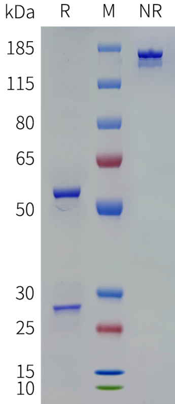
Figure 1. Anti-IL18(camoteskimab biosimilar) mAb on SDS-PAGE under reducing (R) and non-reducing (NR) conditions.
