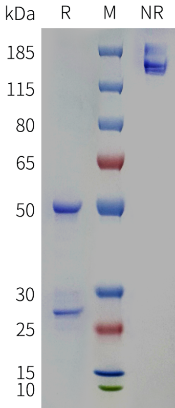
Figure 1. Anti-LRRC32(livmoniplimab biosimilar) mAb on SDS-PAGE under reducing (R) and non-reducing (NR) conditions.
