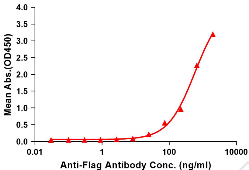
Figure 1. Elisa plates were added with C-Flag&Avi Tag Biotinylated FSHR-Nanodisc (0.2 \mu g/per well) on a Streptavidin pre-coated (0.2 \mu g/per well) plate. Serial diluted anti-Flag monoclonal antibody solutions were added, washed, and incubated with secondary antibody before Elisa reading. From above data, the EC50 for anti-Flag monoclonal antibody binding with Biotinylated FSHR-Nanodisc is 584.7ng/ml.
