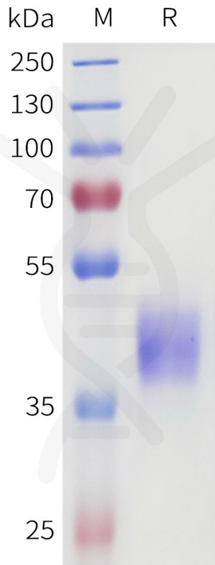
Figure 1. Human 4-1BB(119-160) Protein, hFc Tag on SDS-PAGE under reducing condition.
