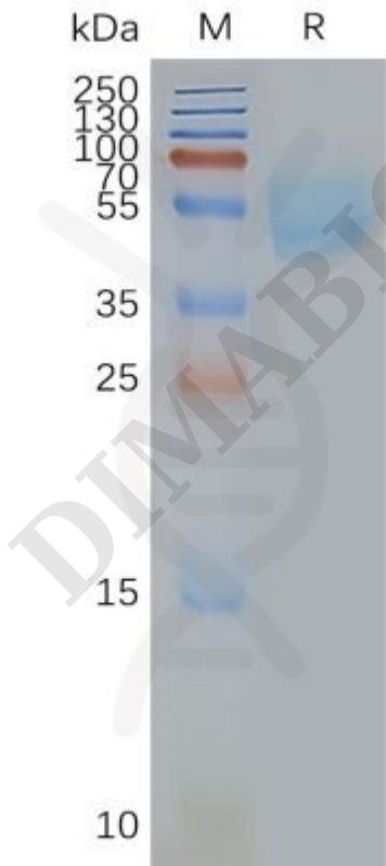
Figure2. Human ADORA2A-Nanodisc, Flag Tag on SDS-PAGE
