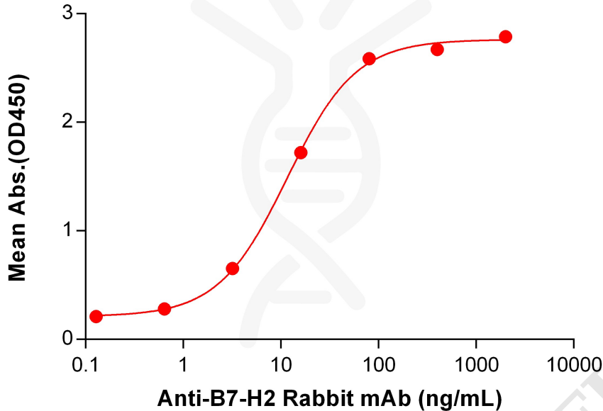
Figure 3. ELISA plate pre-coated by 1 \mu\text{g}/\text{mL} (100 \mu\text{L}/\text{well} ) Human B7-H2 Protein, mFc-His Tag (PME100029) can bind Anti-B7-H2 Rabbit mAb in a linear range of 3.2-80 ng/mL.
