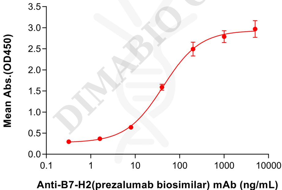
Figure 4. ELISA plate pre-coated by 2 \mu\text{g}/\text{mL} (100 \mu\text{L}/\text{well} ) Human B7-H2 Protein, mFc-His Tag (PME100029) can bind Anti-B7-H2(prezalumab biosimilar) mAb (BME100081) in a linear range of 40-200 ng/mL.
