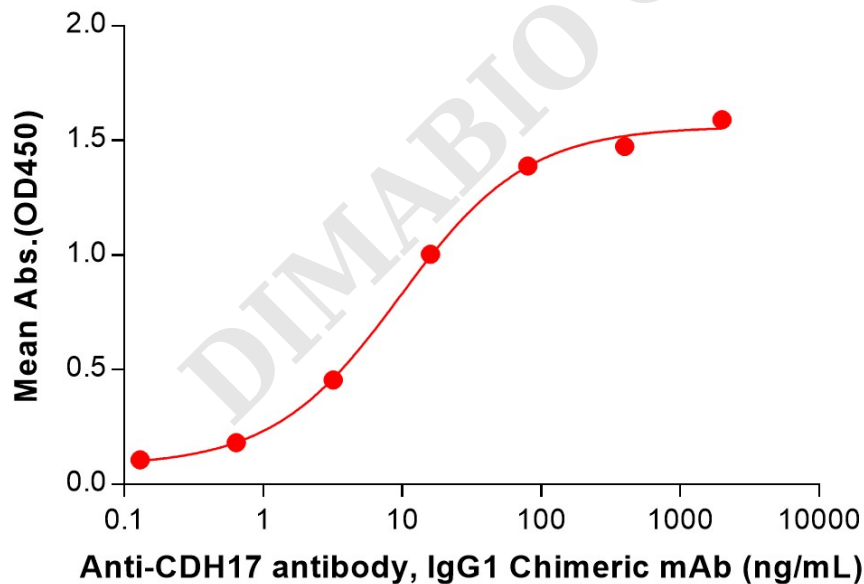
Figure 2. ELISA plate pre-coated by 2 µg/mL (100 µL/well) Human CDH17(245-340) Protein, hFc Tag (PME101564) can bind Anti-CDH17 antibody, IgG1 Chimeric mAb in a linear range of 0.64-80 ng/mL.
