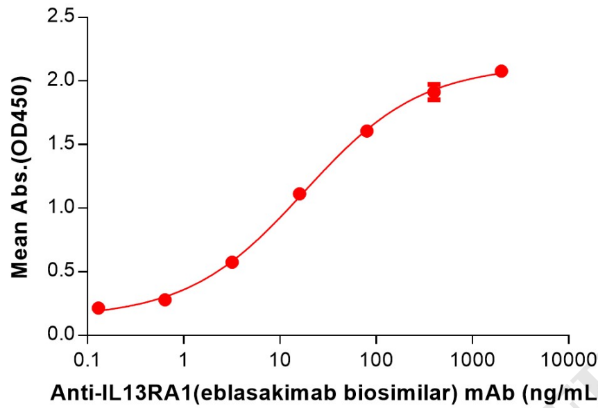
Figure 3. ELISA plate pre-coated by 2 µg/mL (100 µL/well) Human IL13RA1 Protein, His Tag (PME100291) can bind Anti-IL13RA1(eblasakimab biosimilar) mAb (BME100240) in a linear range of 0.64-80 ng/mL.
