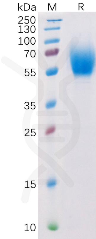
Figure 1. Human IL13RA1 Protein, His Tag on SDS-PAGE under reducing condition.
