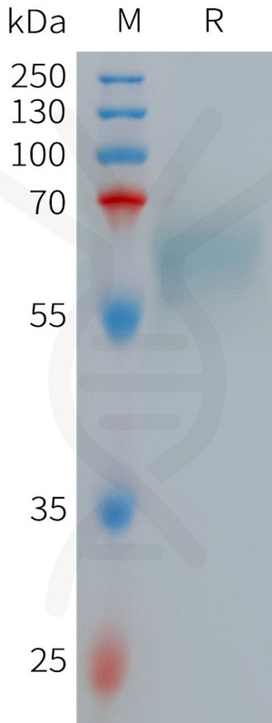
Figure 1. Human LRP10 Protein, His Tag on SDS-PAGE under reducing condition.
