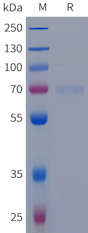
Figure 1. Human LRRC15(1-538) Protein, His Tag on SDS-PAGE under reducing condition.
