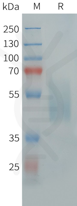
Figure 1. Human NTSR1 Protein, hFc Tag on SDS-PAGE under reducing condition.
