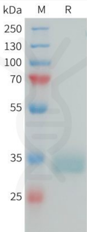
Figure 1. Human PRLR Protein, His Tag on SDS-PAGE under reducing condition.
