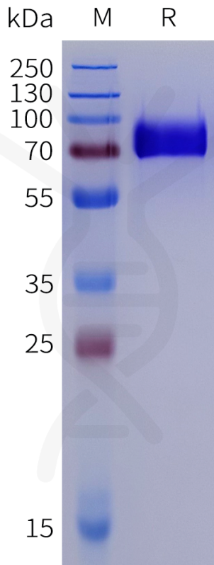
Figure 1. Human SIRP \alpha V2 Protein, mFc Tag on SDS-PAGE under reducing condition.
