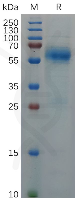
Figure 1. SARS-CoV-2 Nucleocapsid (P13L, E31del, R32del, S33del, R203K, G204R) Protein, His Tag on SDS-PAGE under reducing condition.
